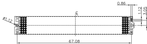
DETAIL C
