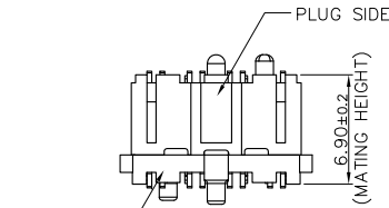
MATING CONDITION
